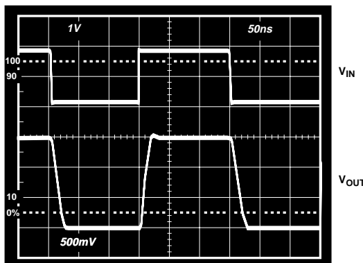
Figure 54. Pulse Response for the Circuit of Figure 52 with +VS = 5 V
